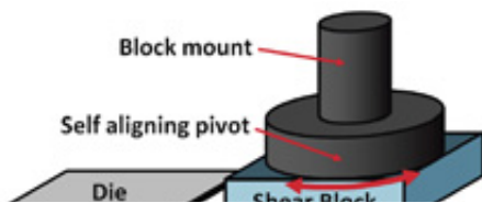
The self-aligning shear tool is designed for forces up to 500kgf
