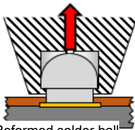
Reformed solder ball
