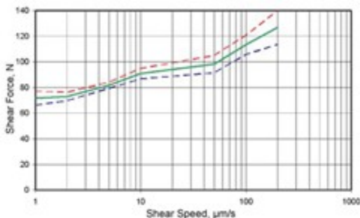
Figure 1 - Influence of shear speed on shear forces of 1206 chip resistors, soldered with SnAgCu To identify the influence on shear result, the test speed was varied in the scope of possibilities of a common Condor 70 shear tester in the range of 1 \mu\text{m/s} to 200 \mu\text{m/s} . Using the example of chip resistors size 1206, the results of this investigation are visible in figure 1.
