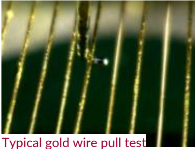
Typical gold wire pull test
