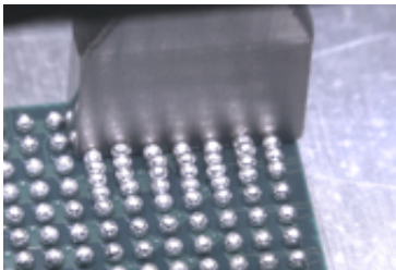
Total ball shear (zone shear) on BGA
