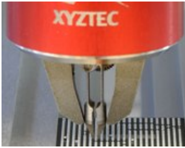
USB Tweezers performing cold bump pull (CBP)
